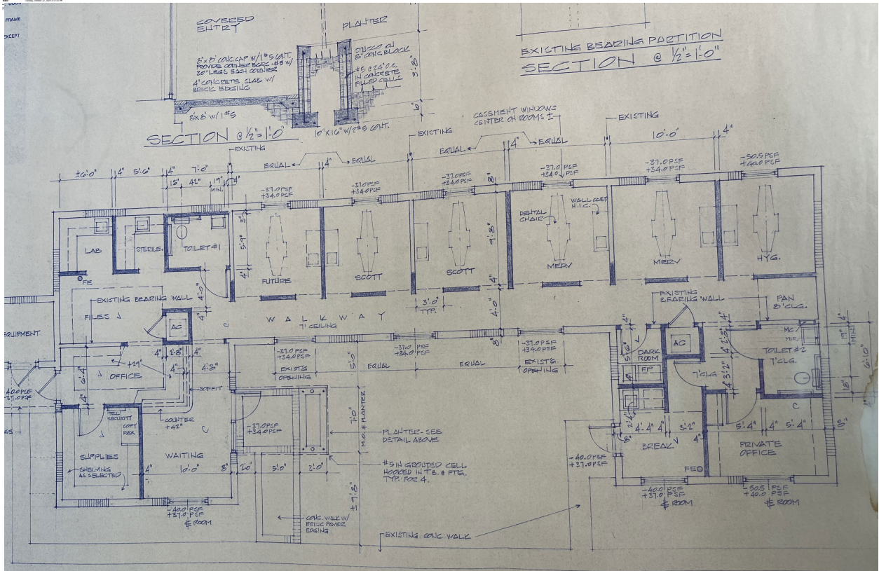
FLOOR PLAN @ 1/4" = 1'-0" OPE - FICE ESTABLISHED
