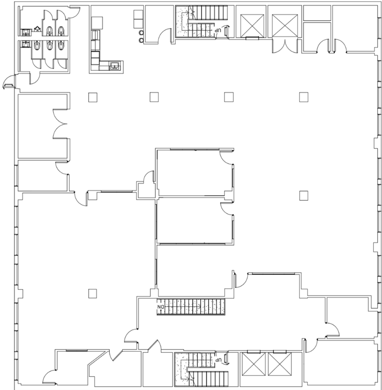
Floor plan
