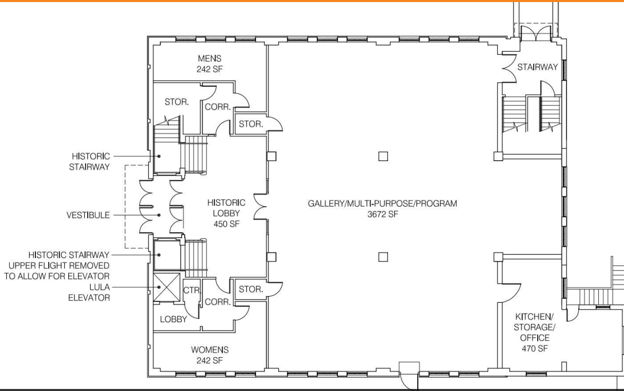
Floor plan provided by Browning Day
