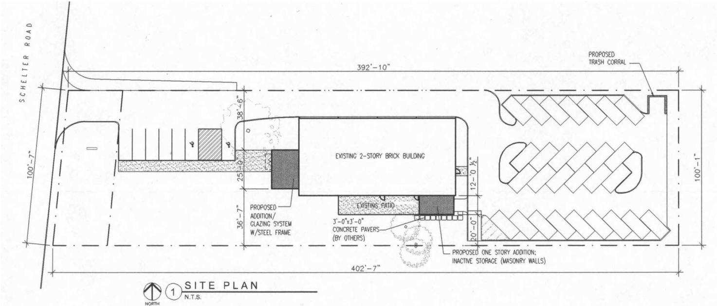
SITE PLAN
