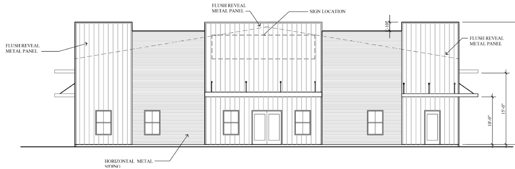
North Elevation
