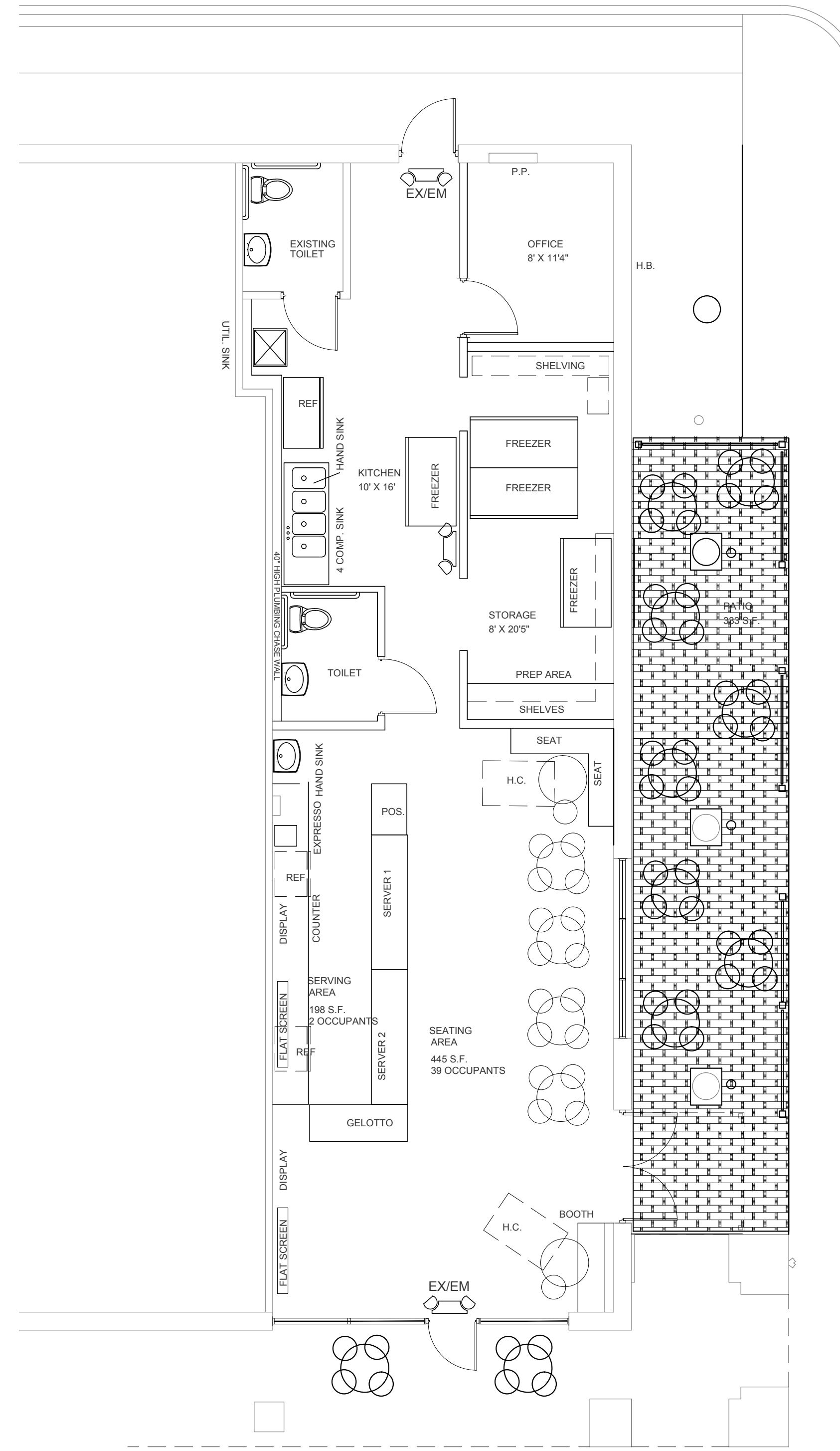
2 A1.1 REVISED FLOOR PLAN SCALE 3/16"=1'-0"
