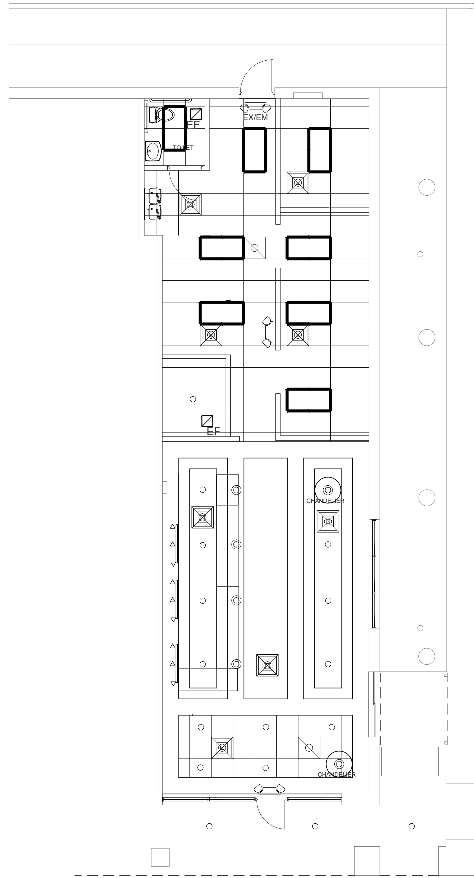
1 A1.1 REVISED REFLECTIVE CEILING PLAN SCALE 3/16"=1'-0"
