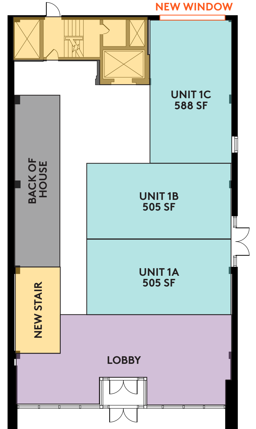
LEVEL 1 FLOOR PLAN
