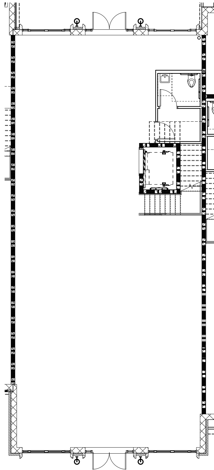
FIRST FLOOR 3 / 32" = 1'-0"
