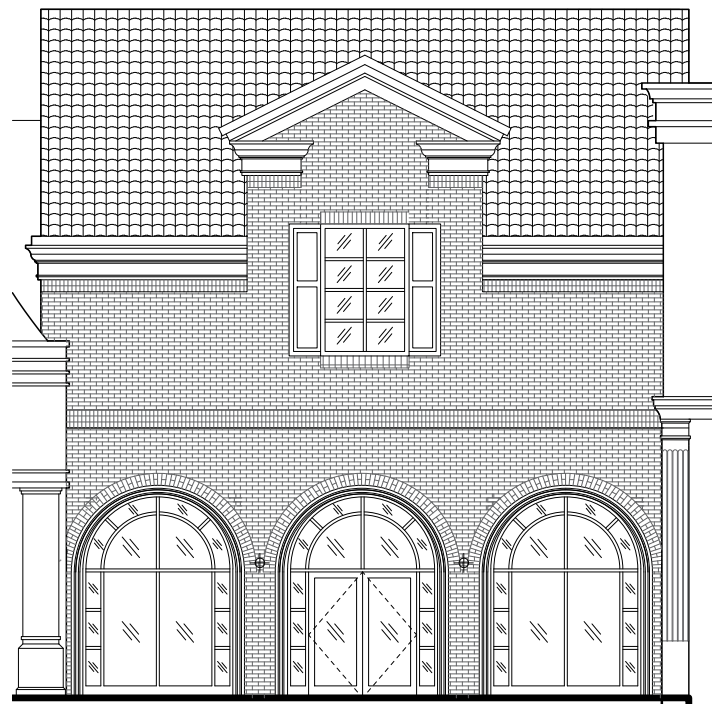
PARKING LOT ELEVATION
