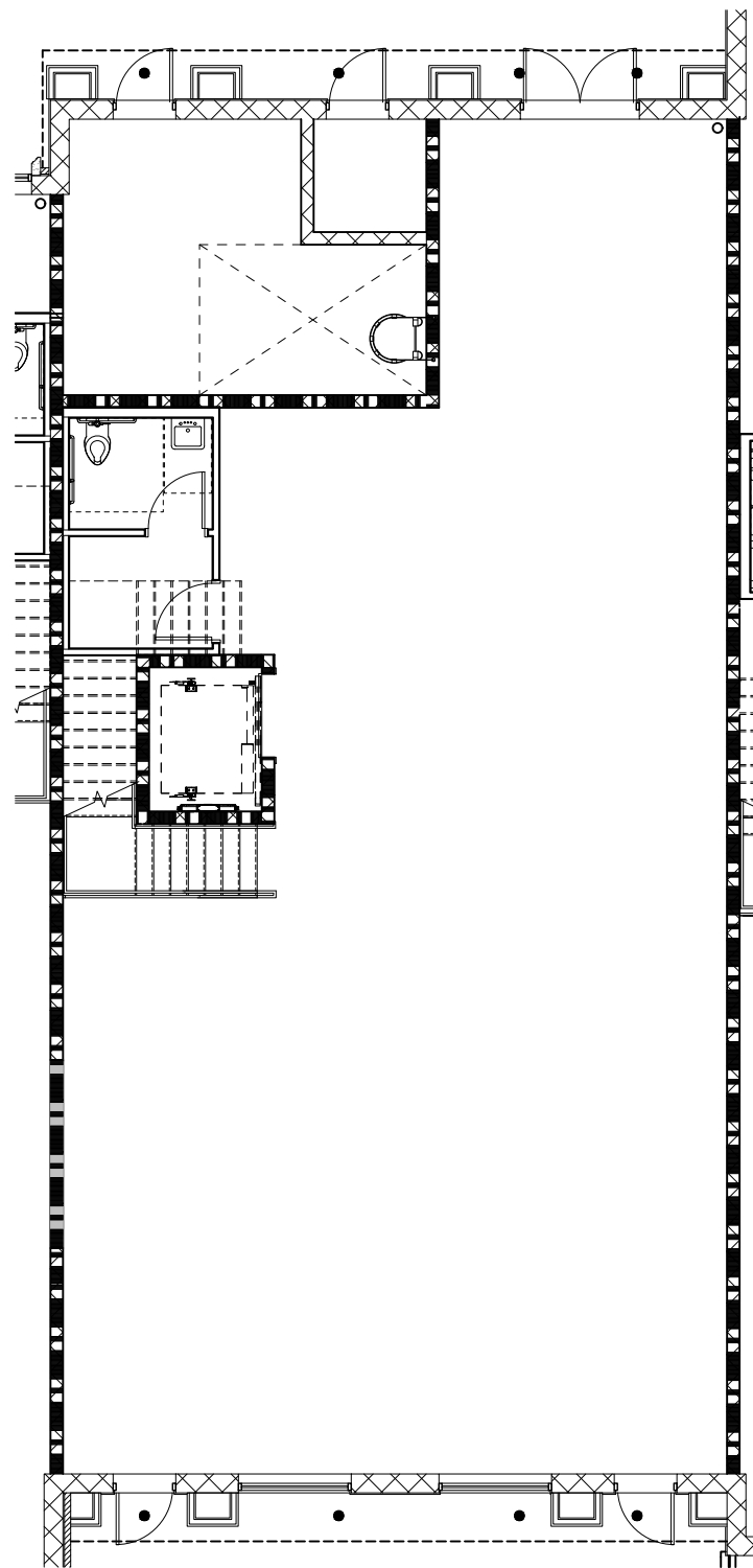
FIRST FLOOR 3 / 32" = 1'-0"
