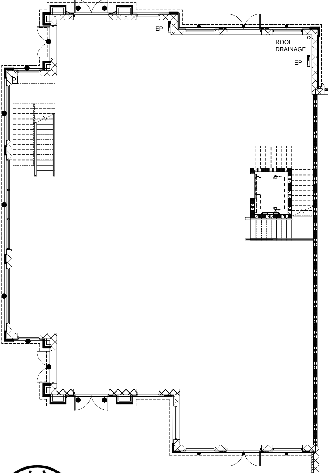
FIRST FLOOR 3 / 32" = 1'-0"
