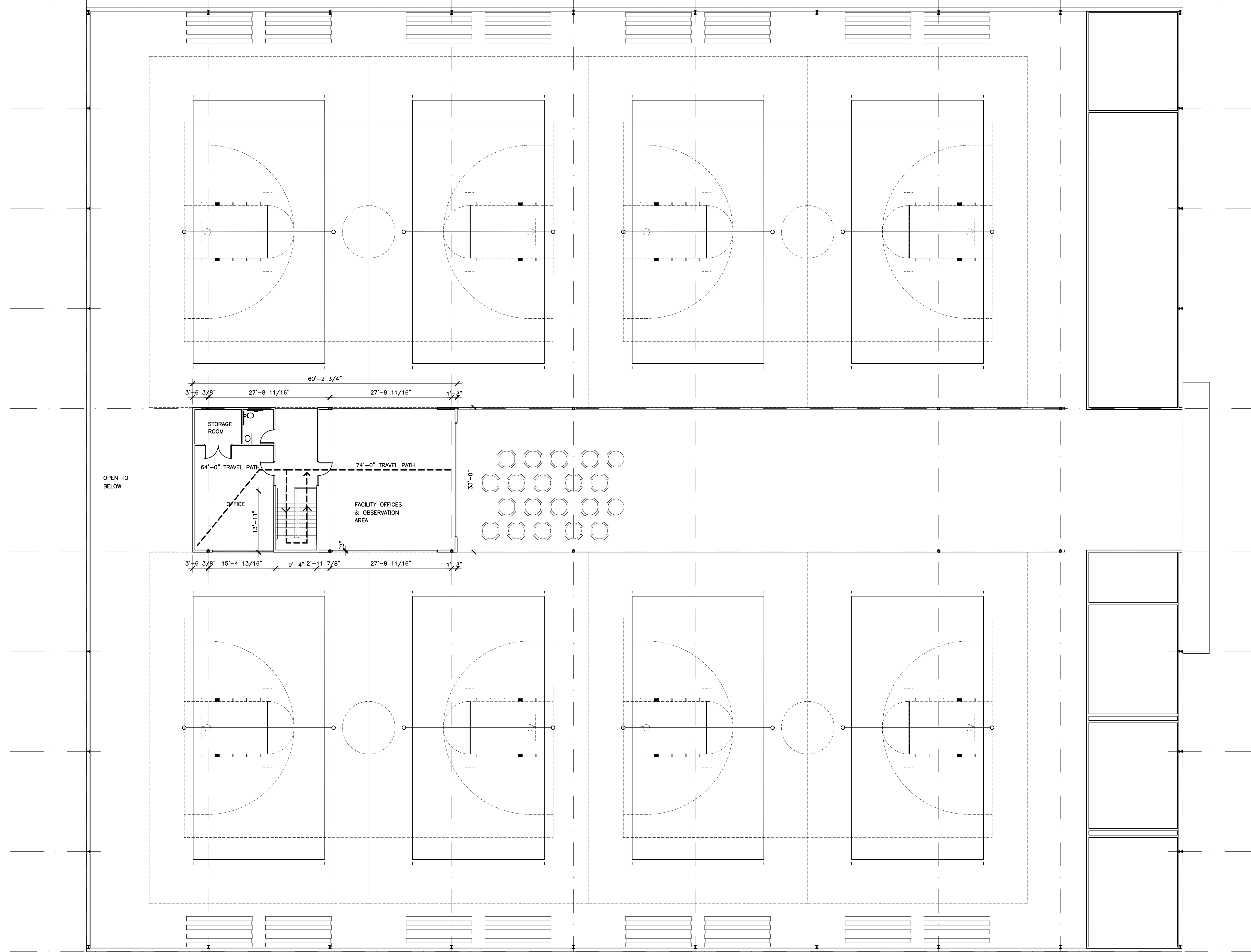
SECOND LEVEL FLOOR PLAN A-2.1 SCALE: 3/32" = 1'-0"
