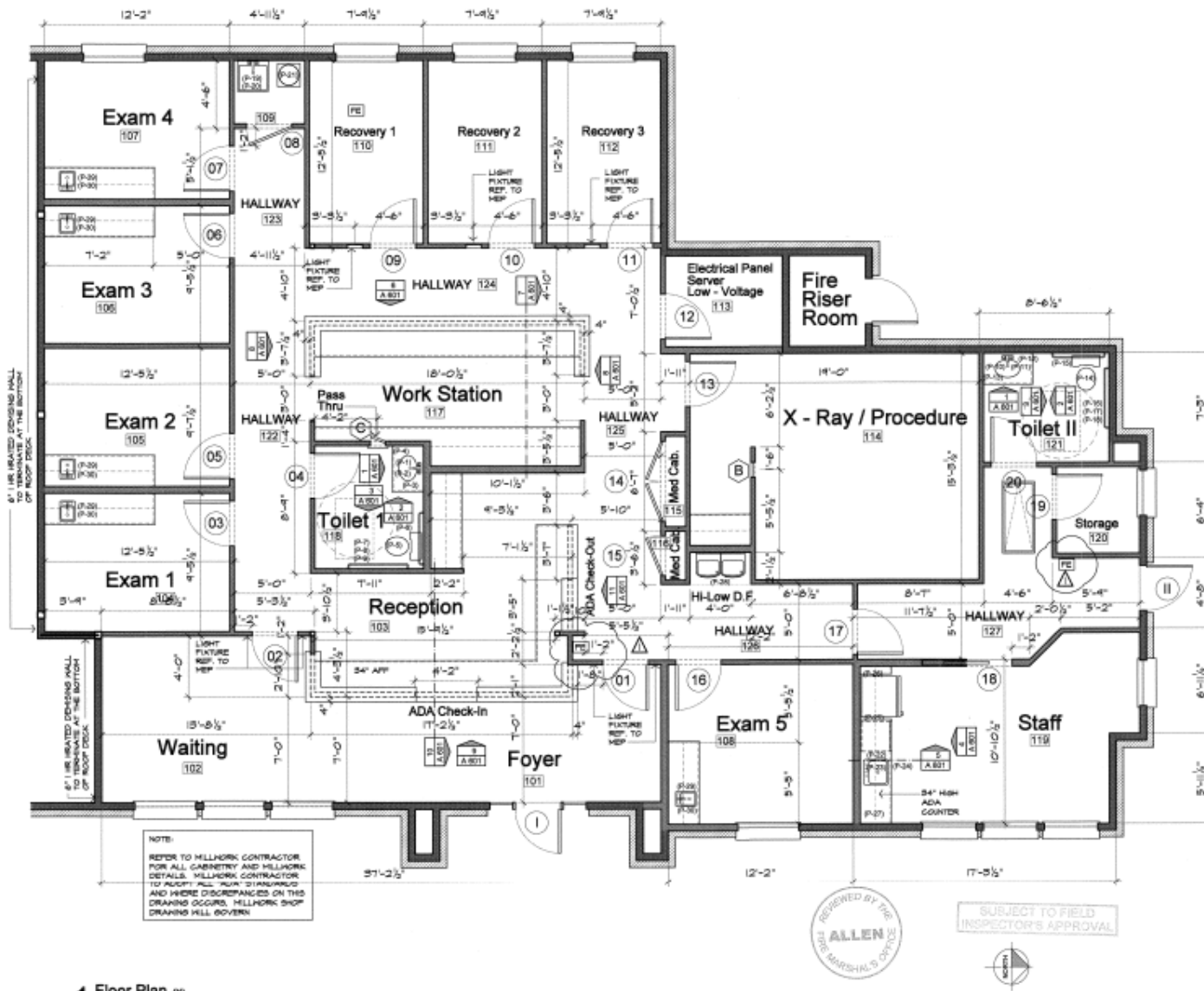
1 Floor Plan (x) SCALE: 1/4" = 1'-0" AREA: 3,198 SQ. FT.
