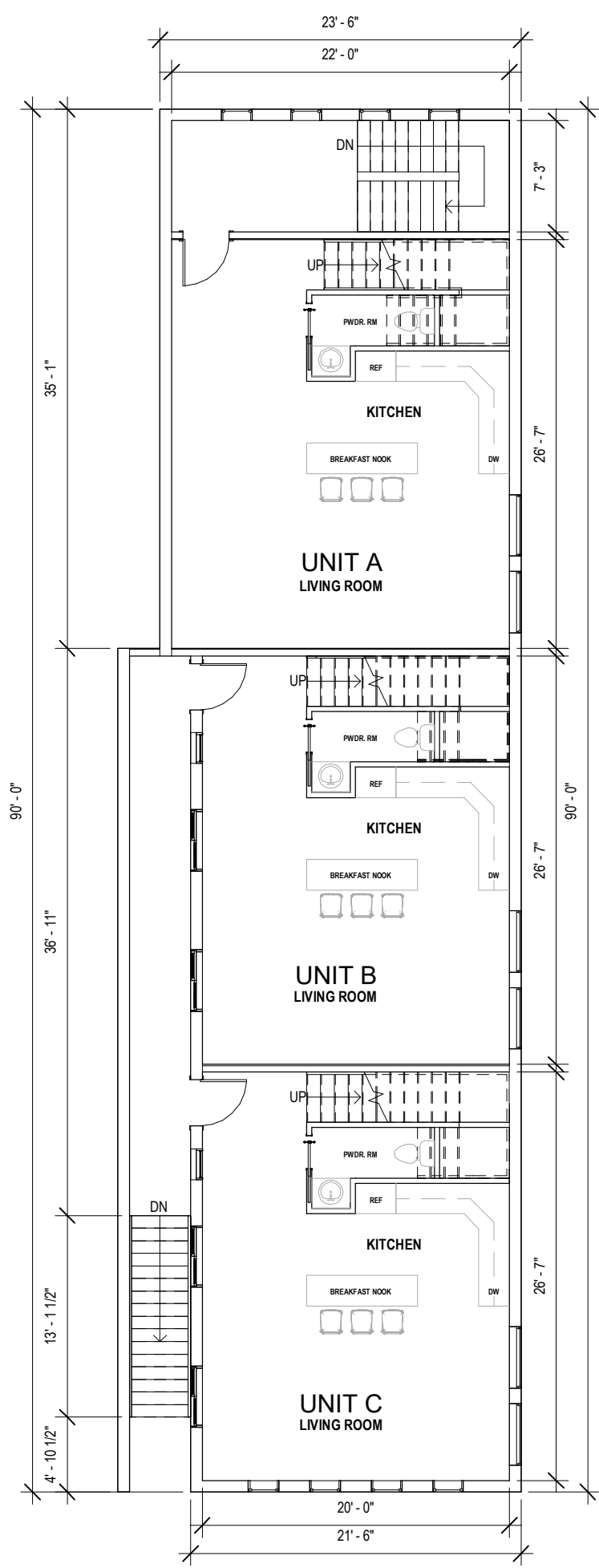
SECOND FLOOR
