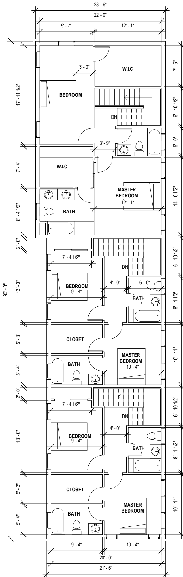
THIRD FLOOR
