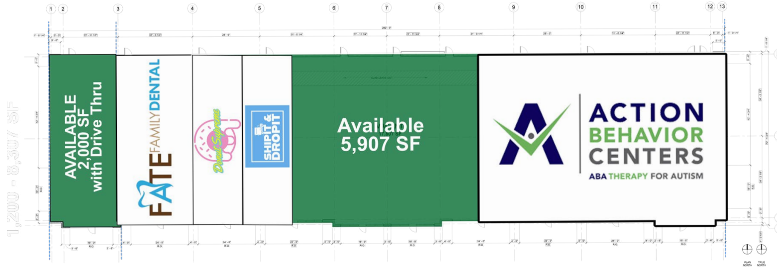
1. FIRST FLOOR PLAN, LOD 1/8" = 1'-0"
