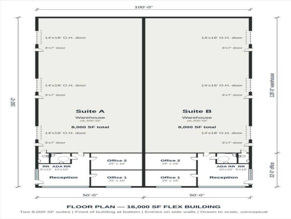
flex-building-16000sf-floor-plan
