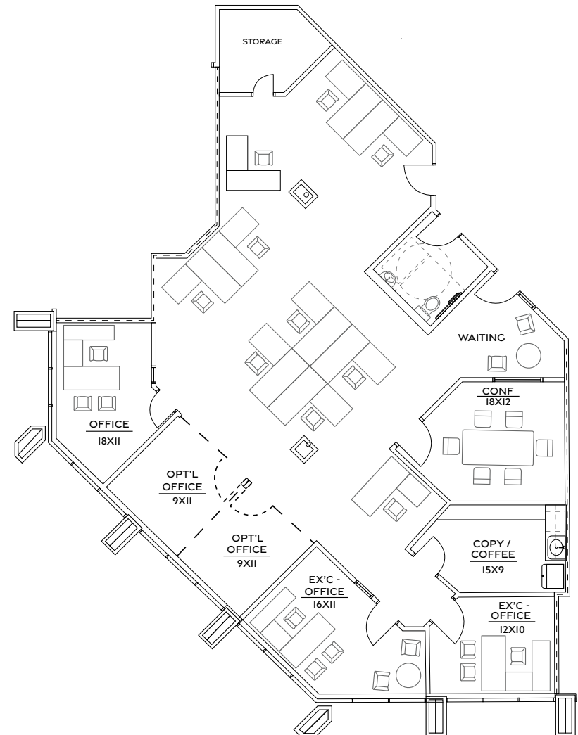
Spec Suite Plan - Option 1
