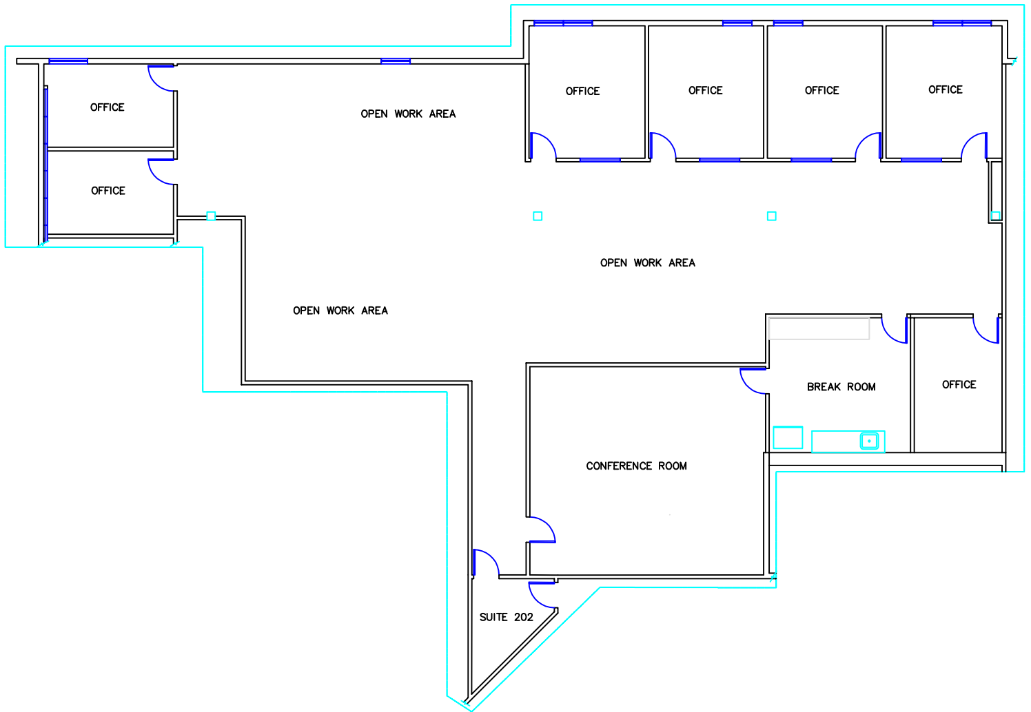
FLOOR PLAN—SUITE 202 SCALE: 1/4"=1'-0"
