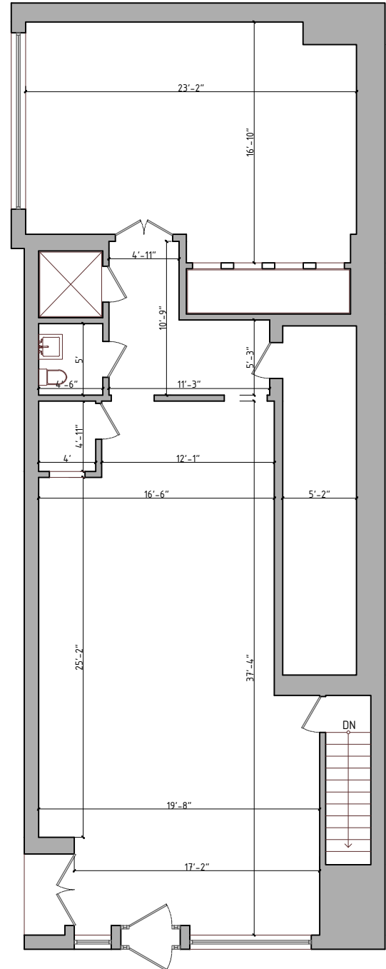
GROUND FLOOR
