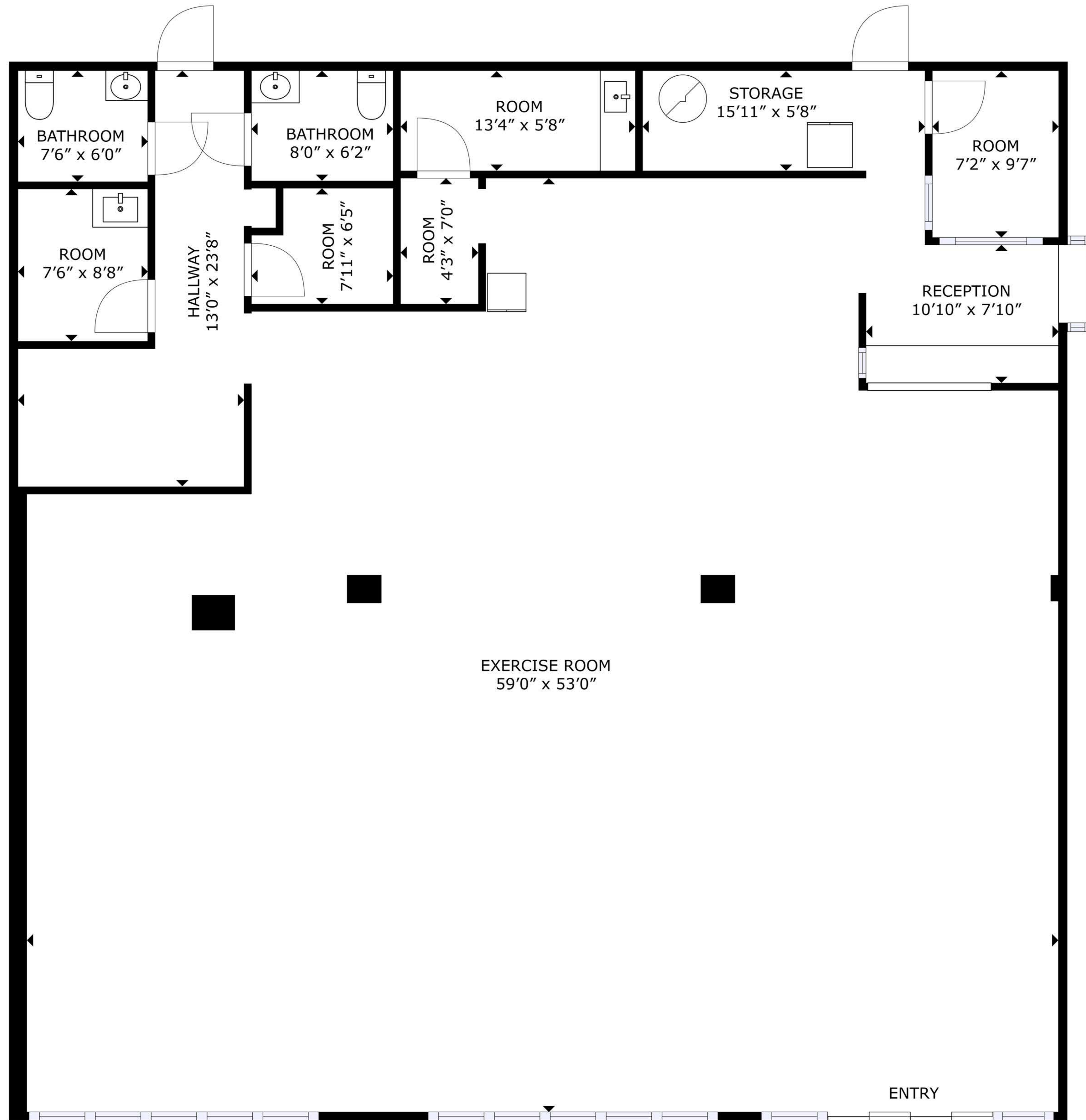
FLOOR PLAN
