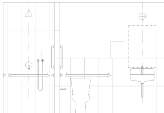
ADA RESTROOM w/ SHOWER
