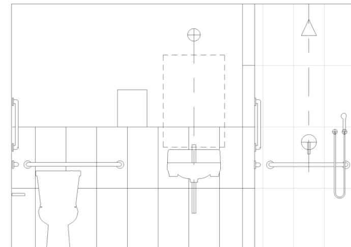
ADA RESTROOM w/ SHOWER
