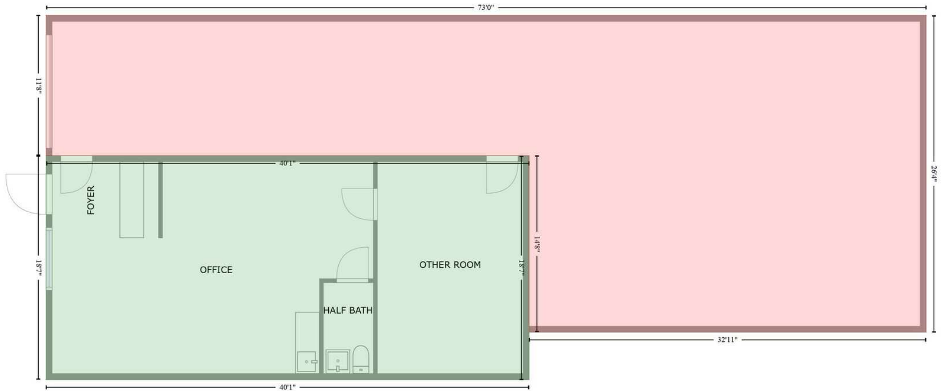
FLOOR 1 [AREA: 745]
