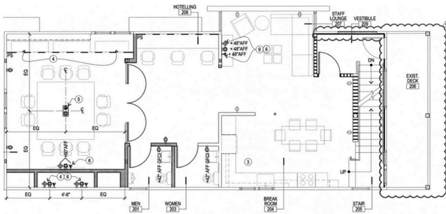
Second Floorplan
