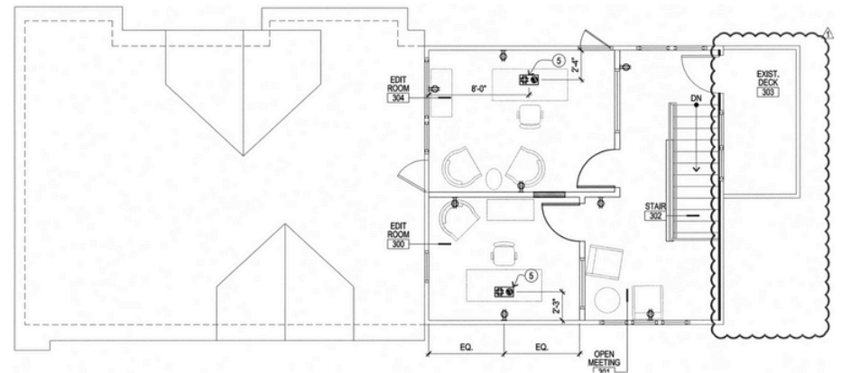
Third Floorplan
