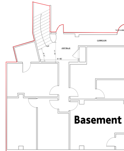
AS-18 FIRST FLOOR BASEMENT PLAN 1/4"=1'-0"
