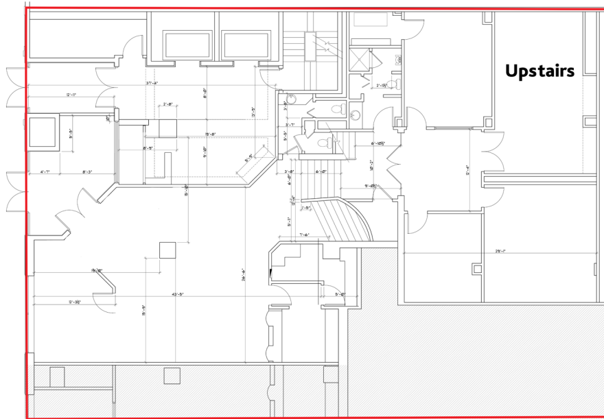
AS-18 FIRST FLOOR PLAN 1/4"=1'-0"
