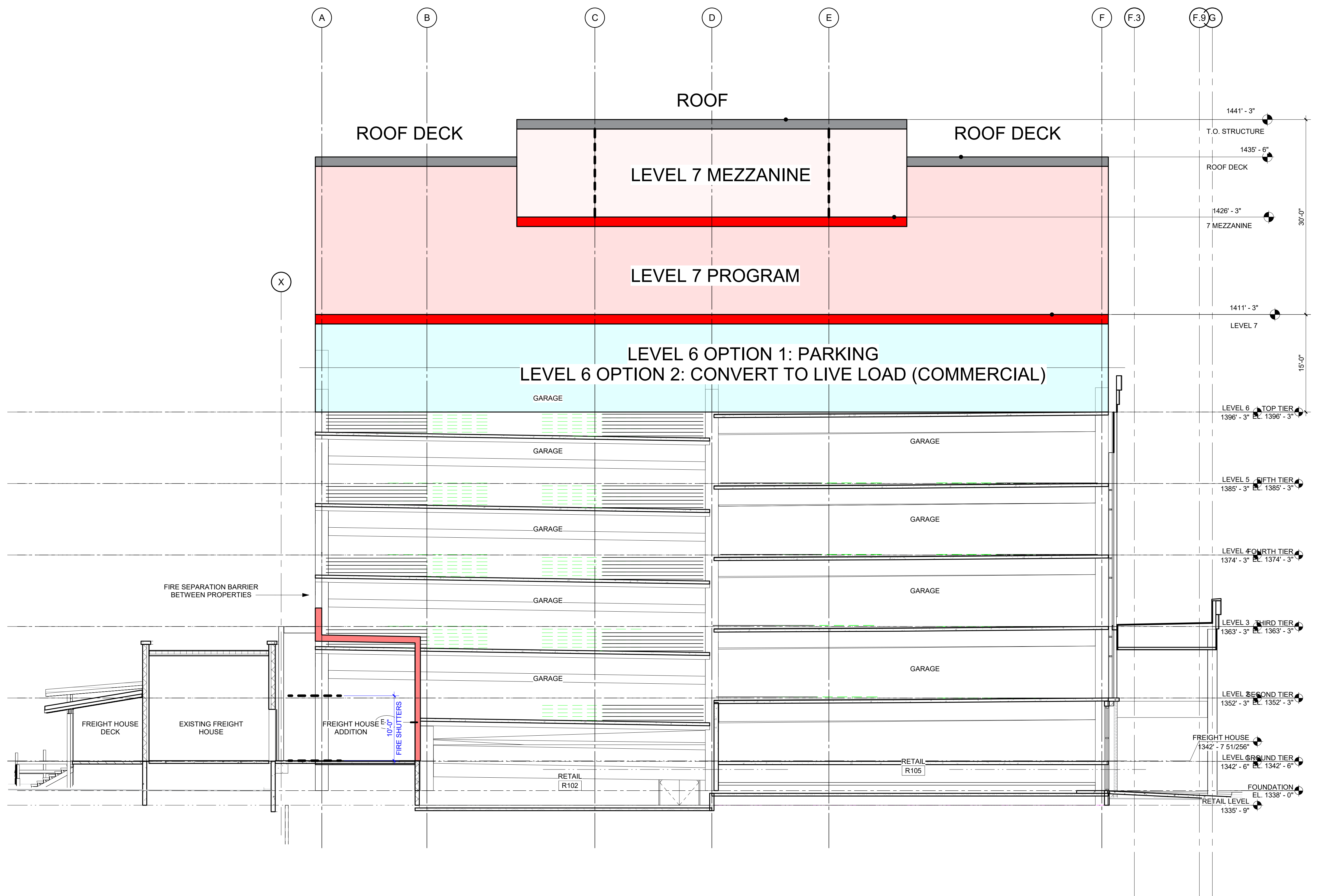
1. Level 7, 7 Mezzanine & Roof Decks Section Diagram scale: 1/8" - 1'-0"
