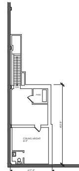
2 SECOND FLOOR RECORD CONDITIONS PLAN SCALE: 1/8" = 1'-0"
