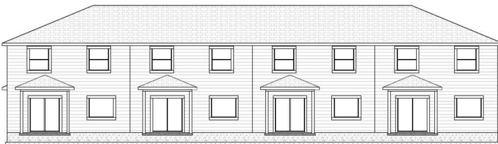
BACK ELEVATION
