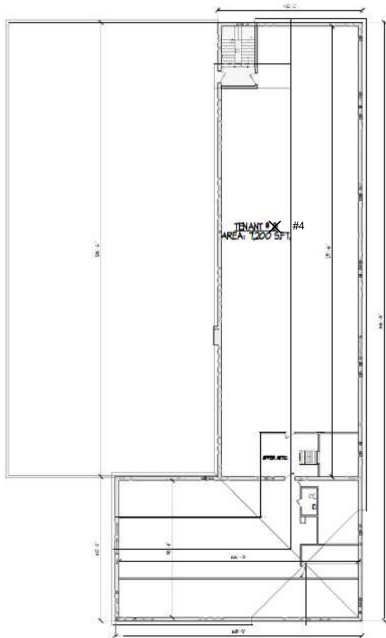
EXISTING ATTIC FLOOR PLAN SCALE: 3/32" = 1'-0" BLDG. GROSS AREA: 1,240 SQ. FT.
