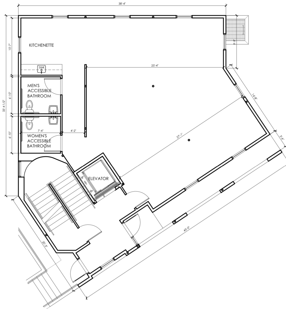
② FIRST FLOOR CONSTRUCTION PLAN 1/8" = 1'
