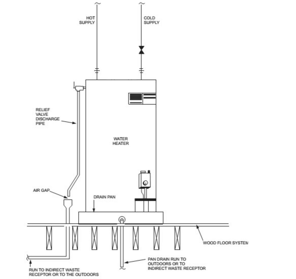
1 A-2 WATER HEATER DETAIL SCALE: 3/16" = 1'-0"
